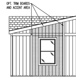
OPTIONAL FRONT ENDWALL W/ ACCENT AREA
